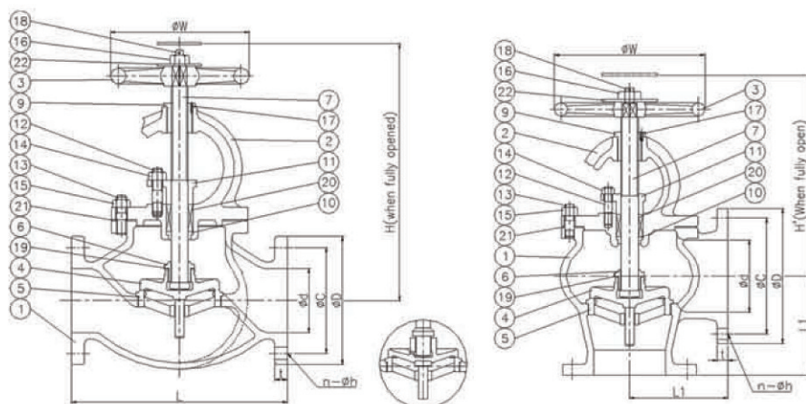
Screw-down check valve
